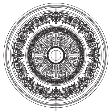
PLAS 826 ACANTHUS ROSETTE 42-3/8"DIAMETER x 3-1/4"DEPTH 4-1/8"DIAMETER AT CENTER HOLE 3-1/4"DEPTH AT CENTER 6-1/4" DIA. FLAT AREA AT CENTER 60 LBS TOTAL WEIGHT
